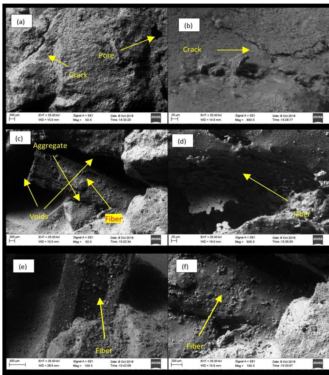
Figure 5: Microscopic characteristics of CTAB - cement paste, aggregate and fiber interaction: (a) and (b) CTAB without fiber; (c) - (f) CTAB with fiber
